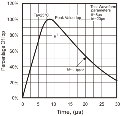
Fig.1 - 8/20μs Peak Pulse Current Wave Form Acc. IEC 61000-4-5
